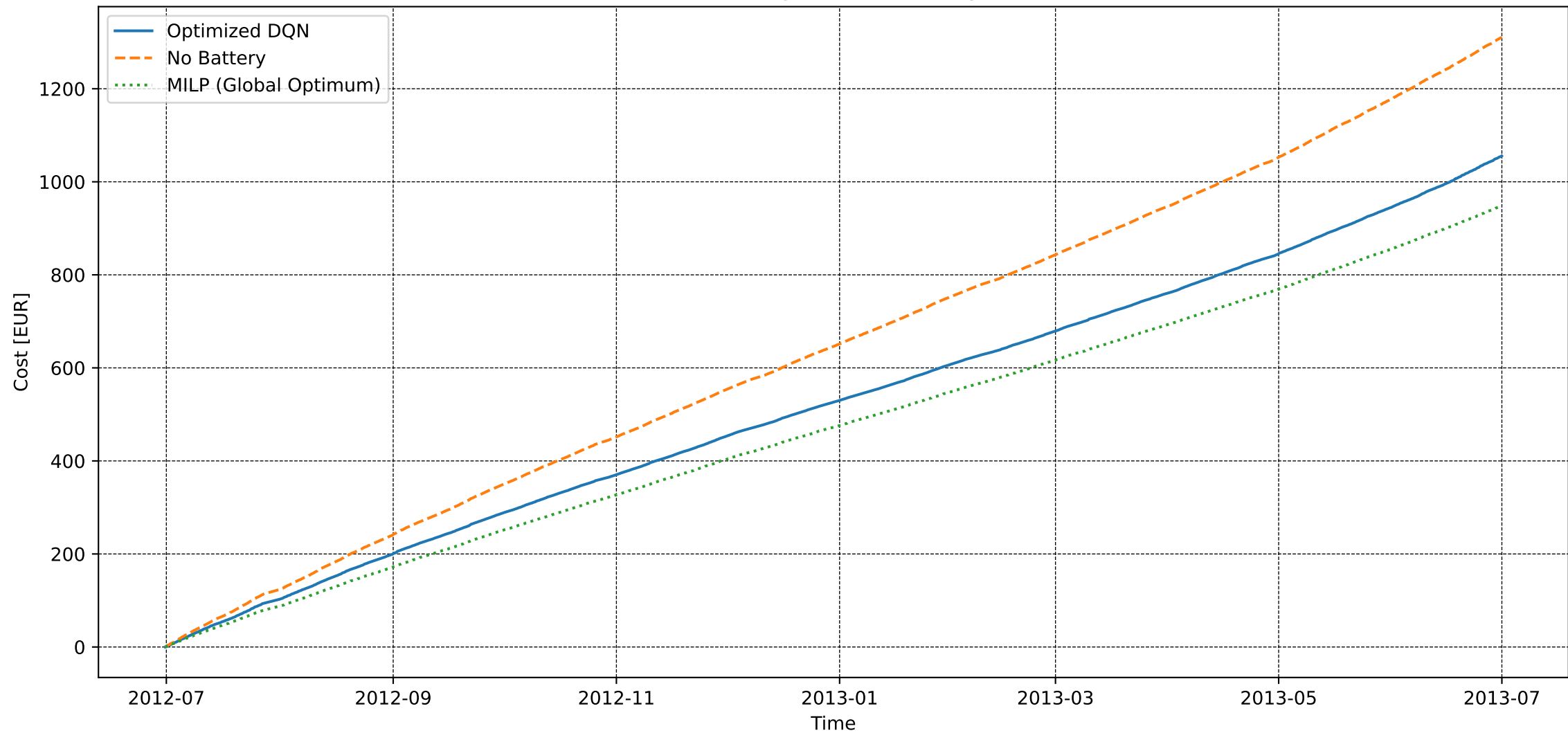
User 113 - Extended Convergence - Electricity Cost [DQN vs MILP]
